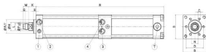
Picture 1 _ unit view
