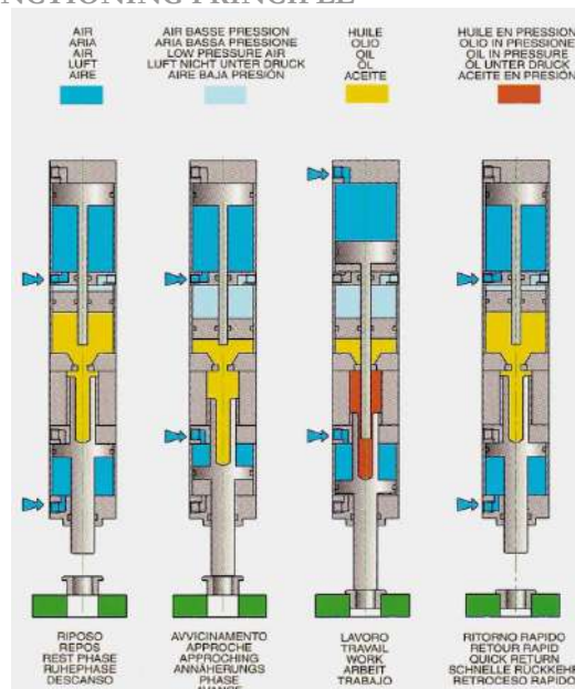
Picture 2 _ functioning principle
